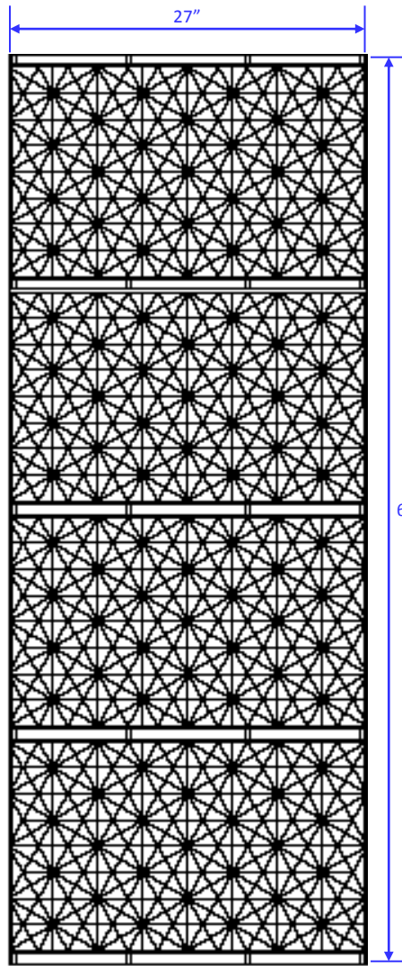
SIDE VIEW
