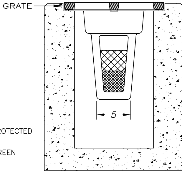
CONCRETE STRUCTURE
