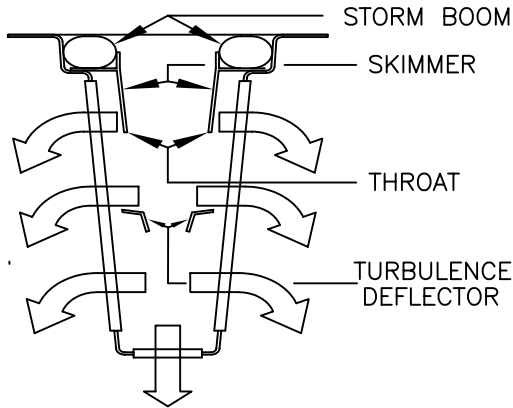
FLOW SCHEMATIC
