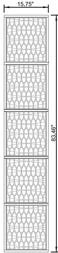
FRONT VIEW
