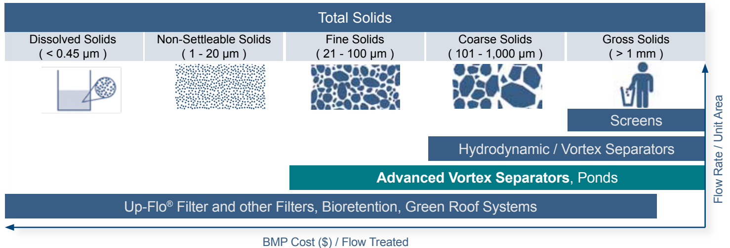
Fig.2 Advanced Vortex Separators treat a broader range of the Total Solids spectrum than conventional hydrodynamic and vortex separators.
