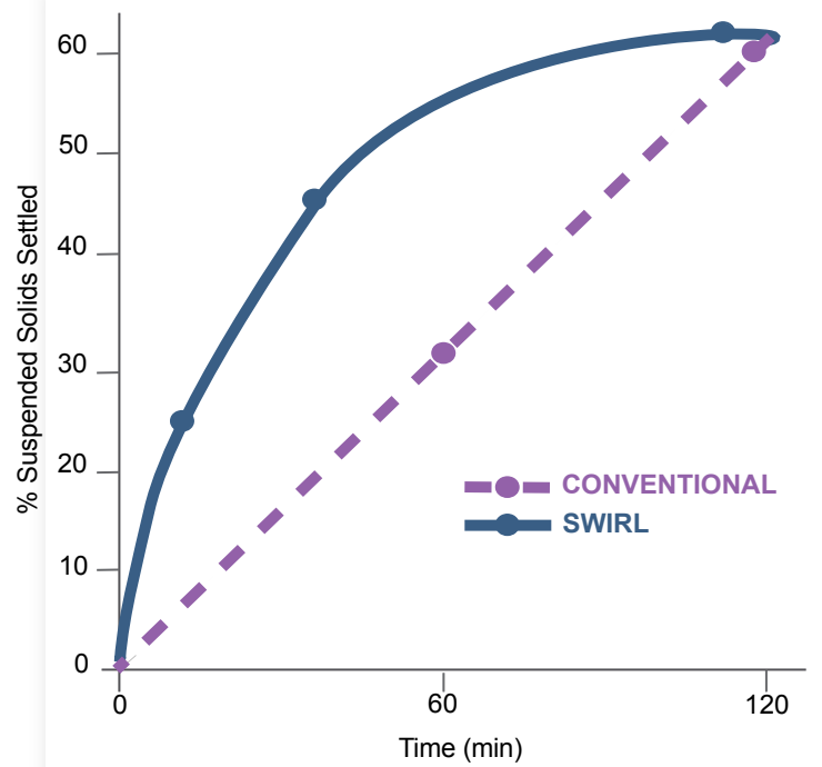
Fig.7 A comparison of time required to capture suspended solids in a swirl separator vs. a conventional sedimentation device, which showed that the bulk of settleable solids settled faster in the swirl separator (Field, 1972).
