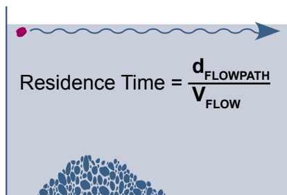
Fig. 14 A particle settles when its residence time within the separator is greater than the time required to settle. Settling time is a function of the distance from the particle to the sump ( d_{\text{SETTLING}} ) and settling velocity ( V_{\text{SETTLING}} ). Residence time is a function of distance from flow inlet to flow outlet ( d_{\text{FLOWPATH}} ) and flow velocity ( V_{\text{FLOW}} ).
