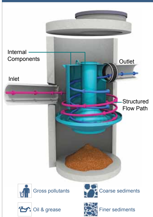
Fig.1 Downstream Defender® Advanced Vortex Separator
