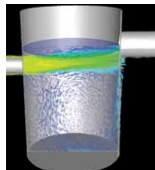
Fig. 15 Fluid modeling shows basic separators are prone to short-circuiting (yellow and green fluid vectors).
