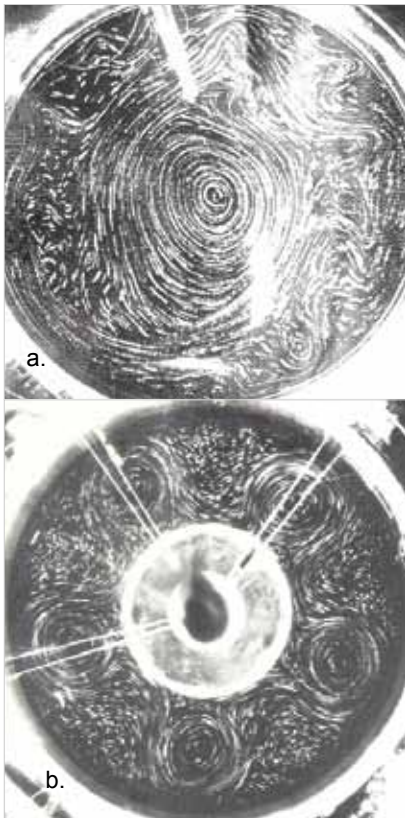
Fig.12 a) A view of the chaotic flow path of a basic vortex separator with no flow-stabilizing components; b) The flow stabilizing components of the Downstream Defender® minimize turbulence over a wide range of flows to increase settling performance and minimize headloss.
